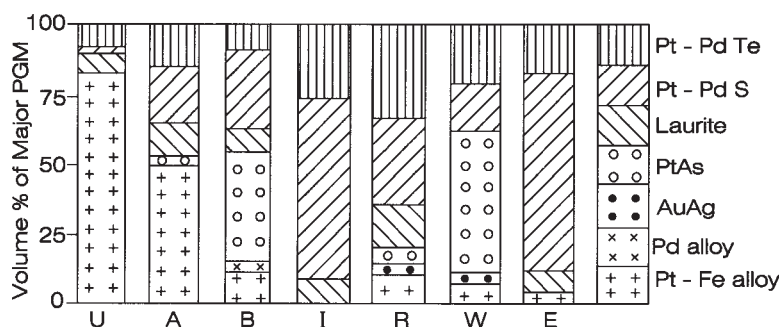
FIG. 9. PGM distribution for the Merensky Reef at all mines in the western limb, and the Lebowa mine in the eastern limb (denoted E). Other abbreviations as in Figures 3 and 7. Data from mining company reports, summarized by Schouwstra et al. (2000), and an unpublished report from Impala mine.
