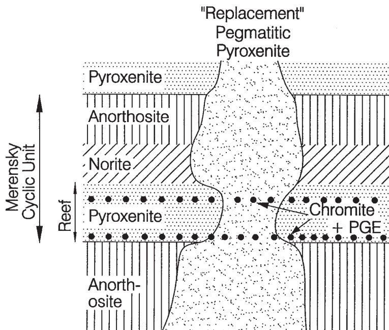
FIG. 12. Schematic representation of the observations regarding the preservation of PGE mineralization and chromite in their original location in the reef even after extensive replacement of the silicate host by a discordant ultramafic body (Viljoen et al. 1986b).
