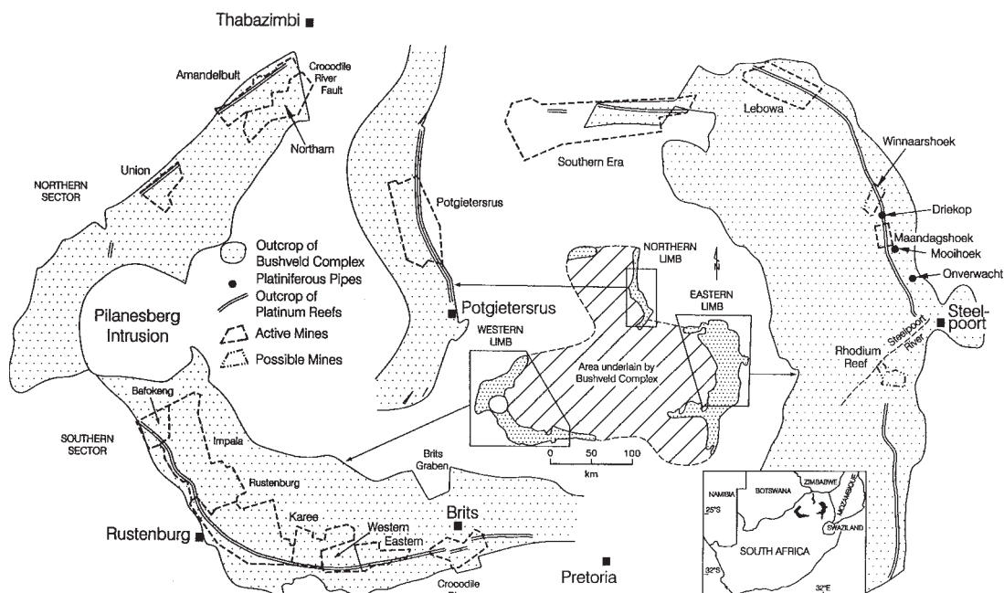
FIG. 1. General map of the Bushveld Complex (center), with different limbs (exploded views) showing active and proposed mines on Merensky or UG2 chromitite reefs (or both). PGE reefs are shown as a double line. The platiniferous pipes also are shown.
