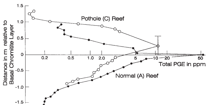
FIG. 10. Example of vertical distribution of the PGE from two sections across A (normal) and C (pothole) Merensky reef at the Impala mine, shown by solid and open symbols respectively. Continuous sampling every 10 cm is employed, except in the pothole reef, where the entire 60 cm-thick pegmatitic pyroxenite is taken as a single sample. Note log scale for PGE content. Data given in Table 3.
